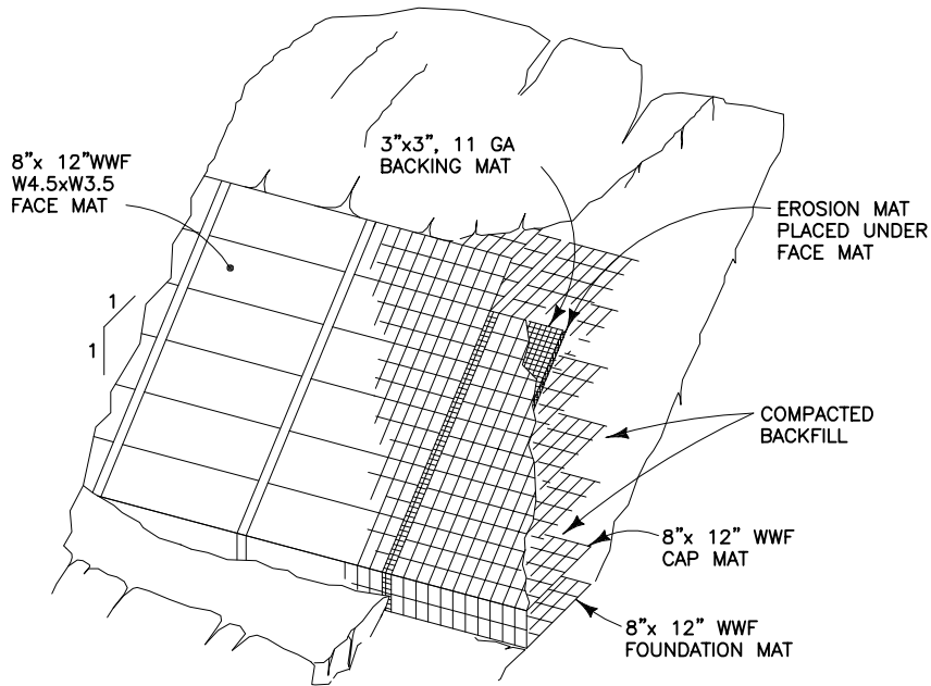
PICTORIAL ELEVATION
